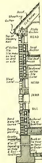
Wall Section
